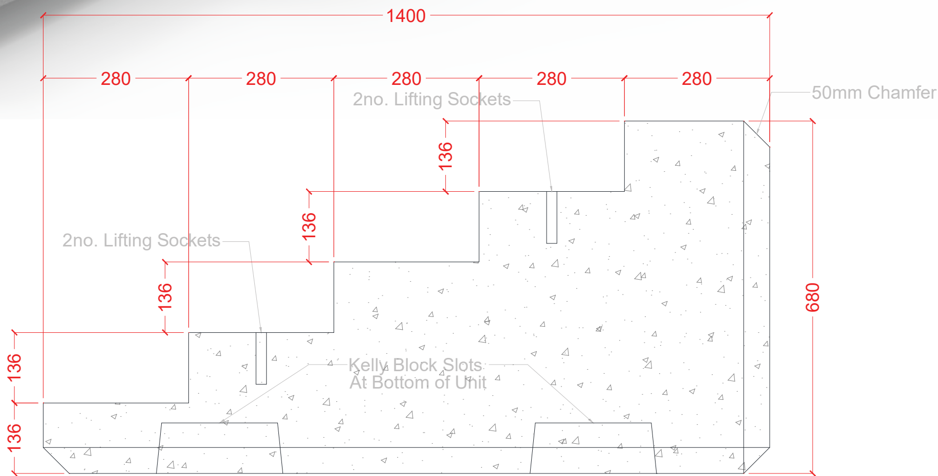
SIDE ELEVATION 2
