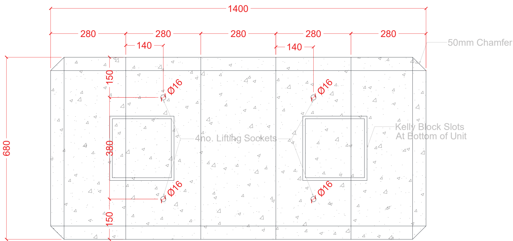
PLAN
