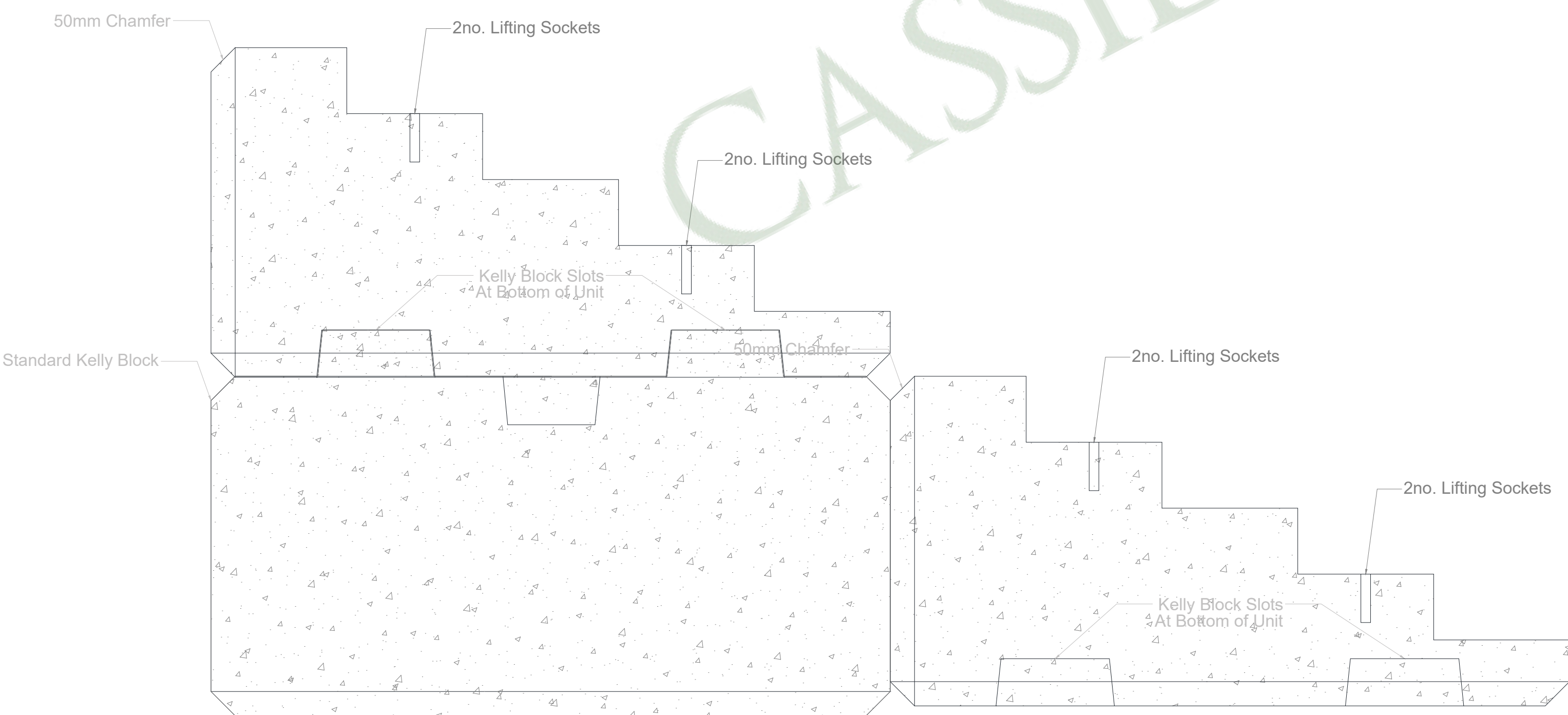
SIDE ELEVATION 1
