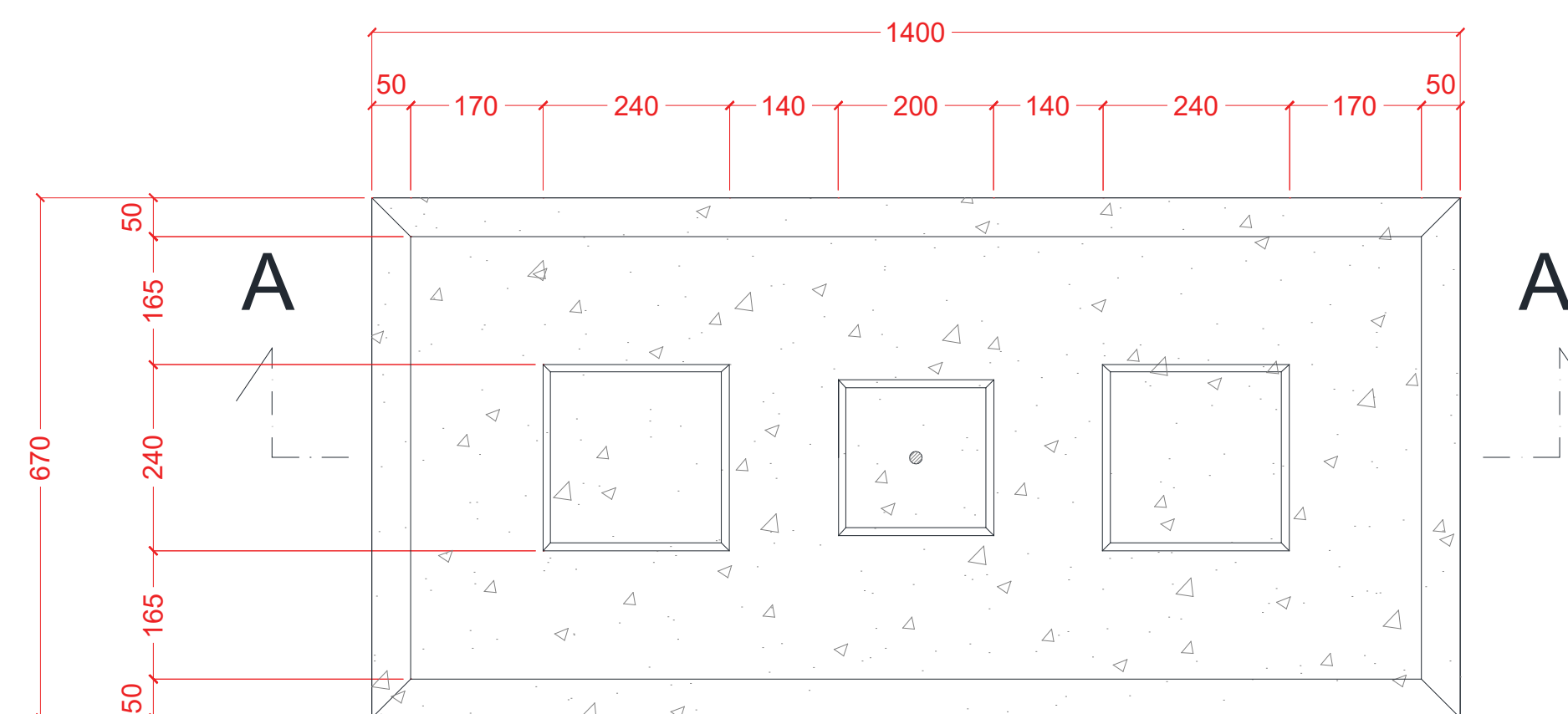
PLAN
