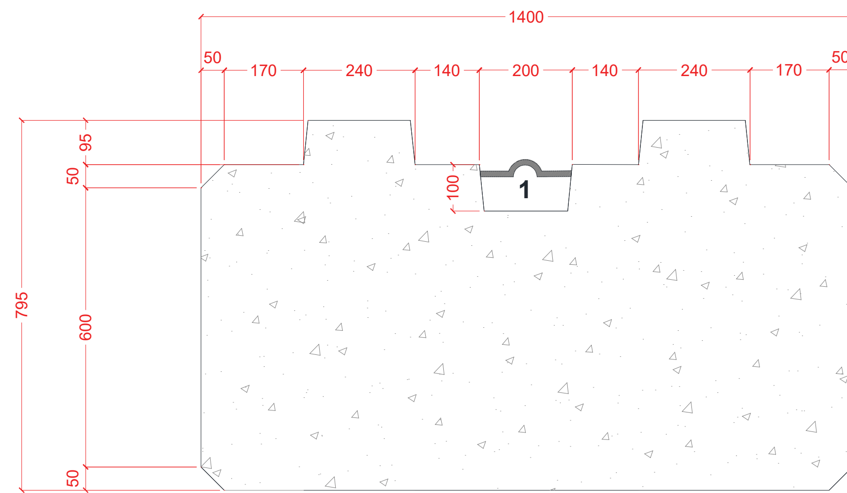
FRONT ELEVATION
