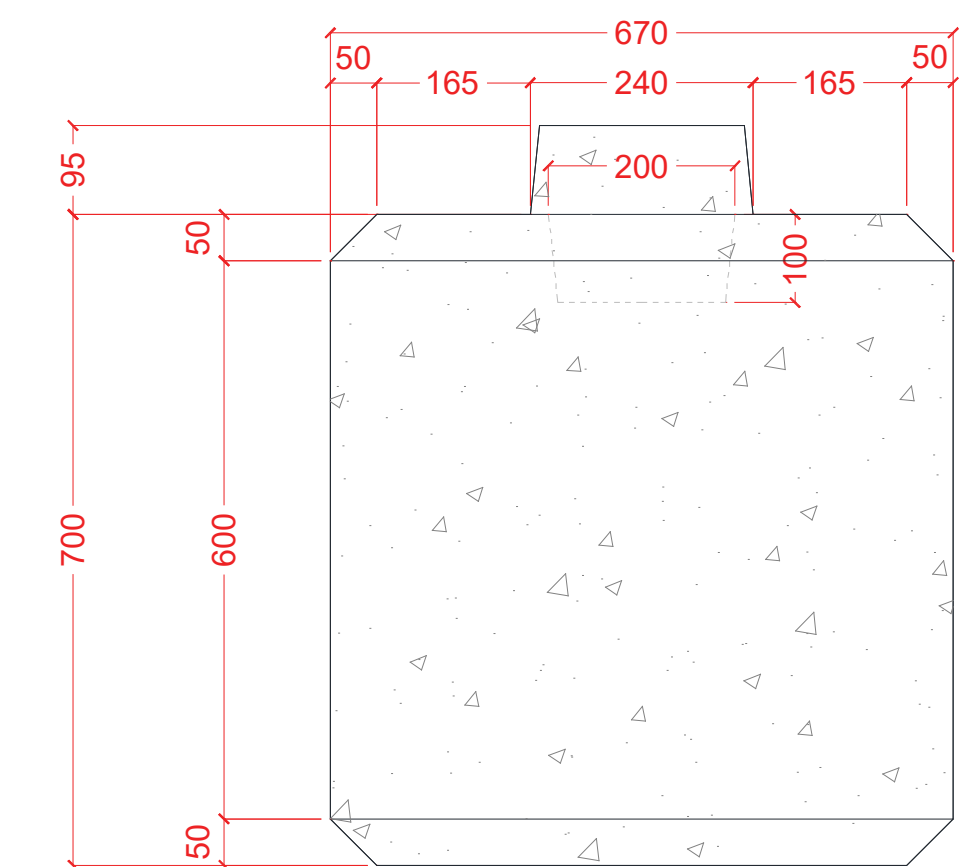
SIDE ELEVATION
