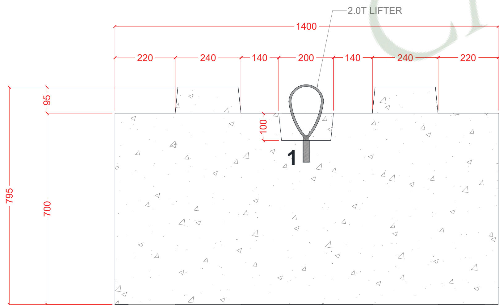
FRONT ELEVATION
