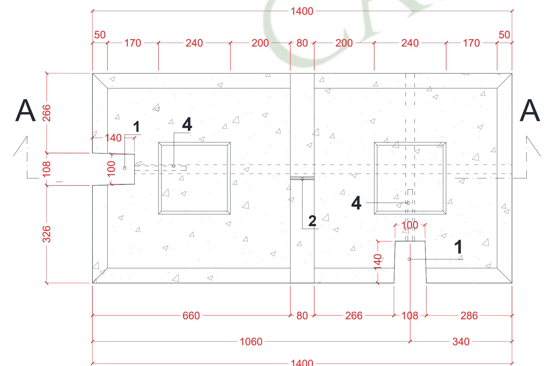
PLAN
