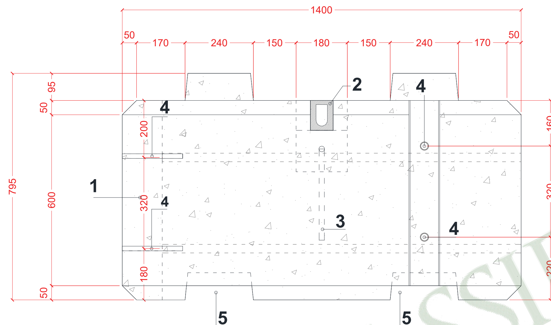
FRONT ELEVATION
